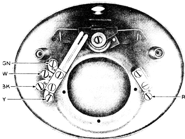
FIG. 5—D1-3 HANDSET MOUNTING
