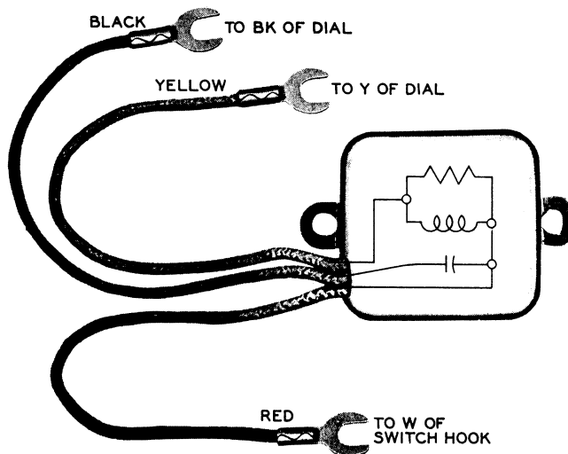
FIG. 6—61N FILTER CONNECTIONS
